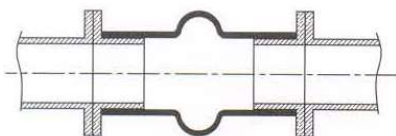
AXIAL CONTRACTION
