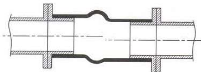
LATERAL DEFLECTION
