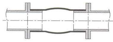
AXIAL EXPANSION
