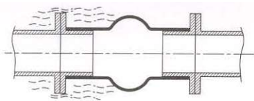
VIBRATION ISOLATION
